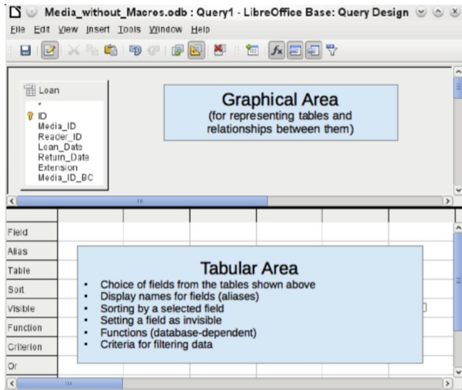
Figure 74: Areas of the Query Design dialog
