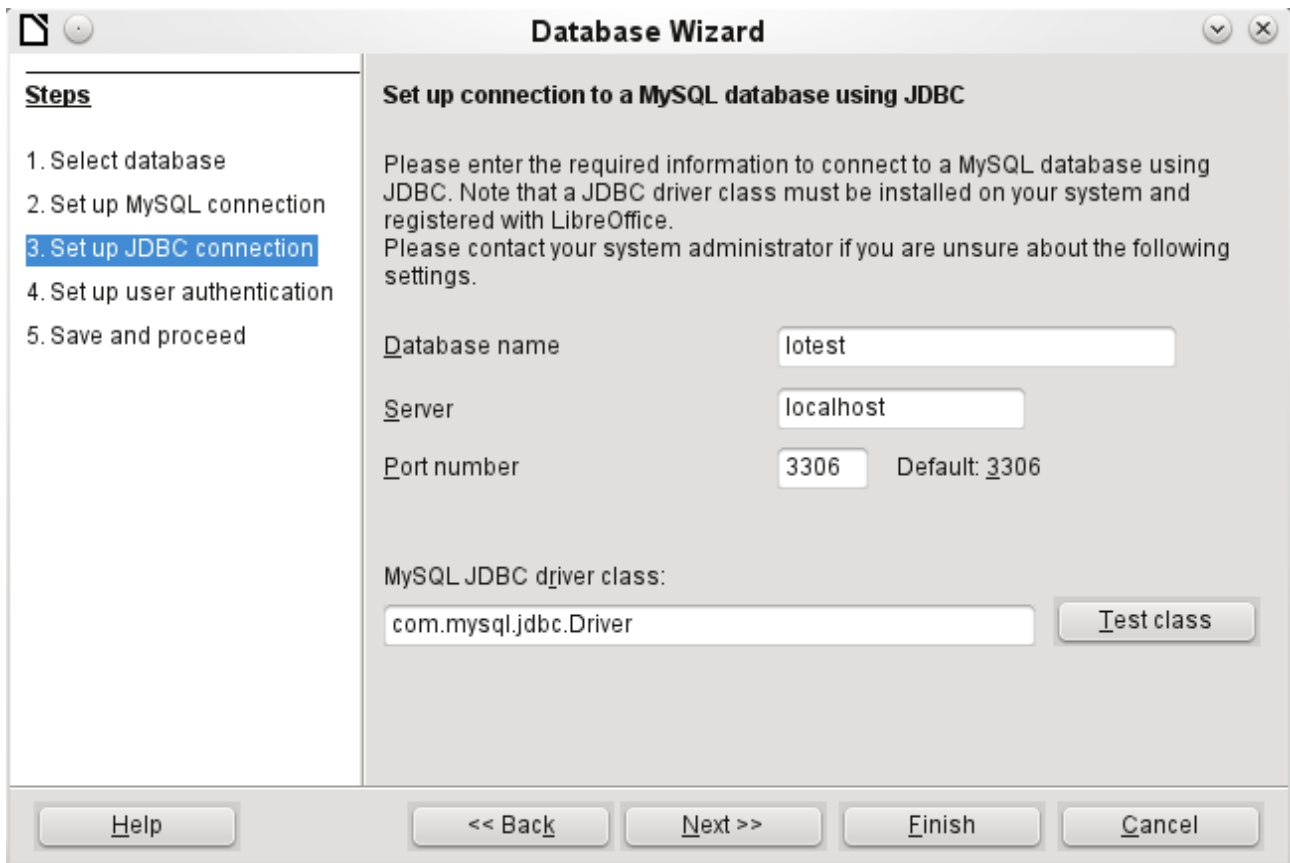
Figure 22: Setting up a connection using JDBC
